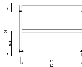
Leuningframe RS TOWER 4 & 5
