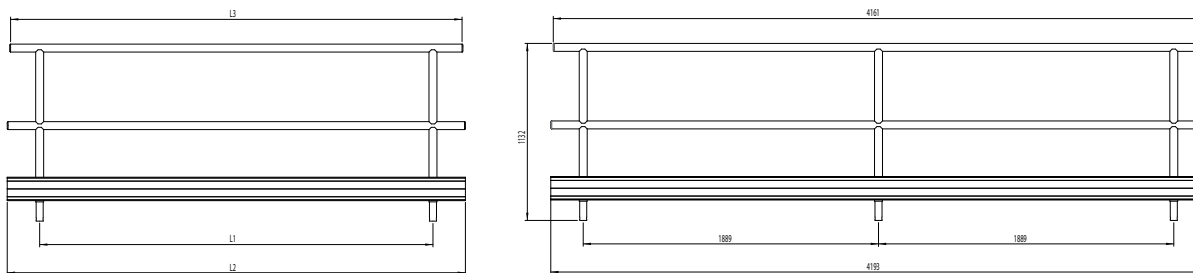
331524 Guardrail frame DRB 4m
